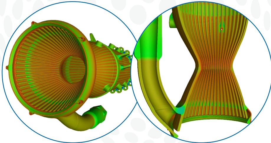
3D CT Scan of an Additive Manufactured Rocket Engine
